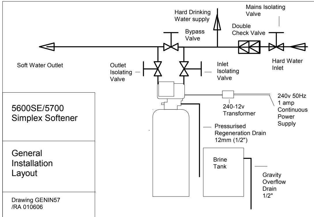
Fig 1 General Installation Layout 5600SXT Simplex Scavengers
